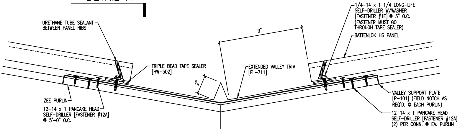
DETAIL A
