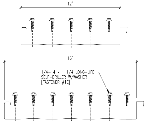
FASTENER LOCATIONS
