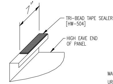
HIGH EAVE SEALANT DETAIL
