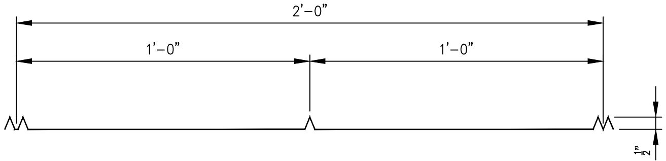
5V Crimp Panel Profile
