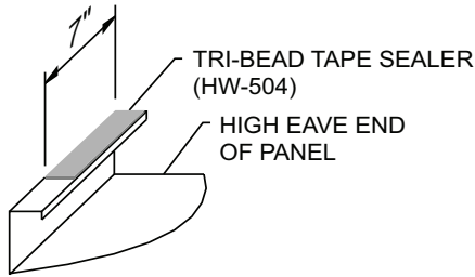
HIGH EAVE SEALANT DETAIL
