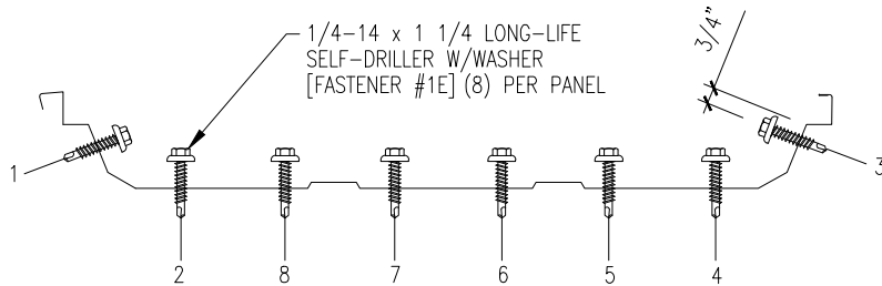
FASTENER SEQUENCE @ EAVE
