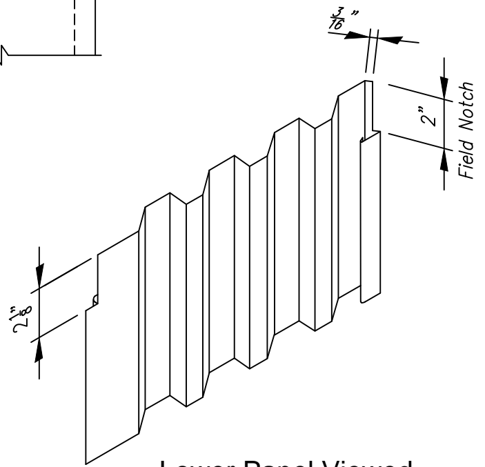
Lower Panel Viewed From Interior Side
