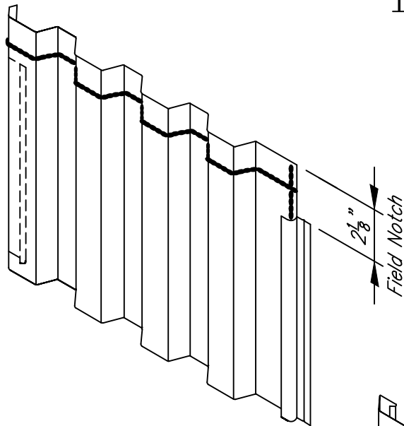
Lower Panel Viewed From Exterior Side
