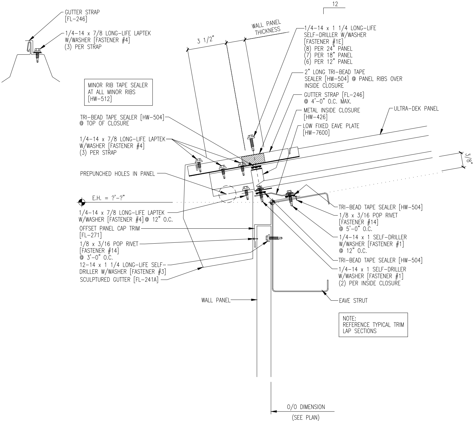
FASTENER SEQUENCE @ EAVE
