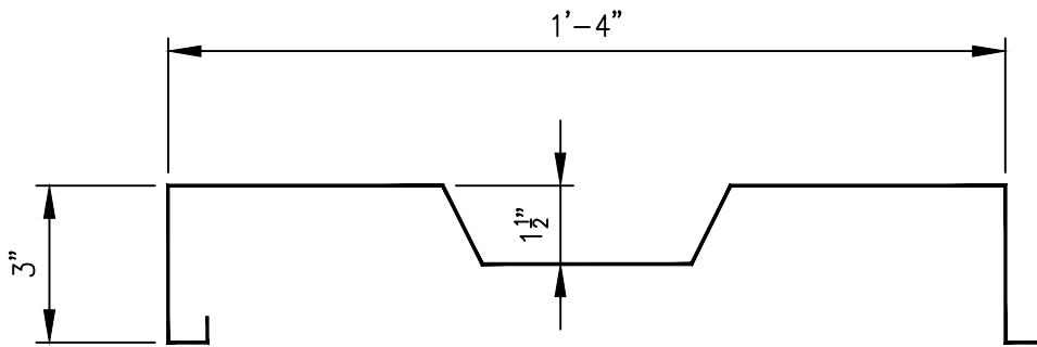
ShadowRib Panel
