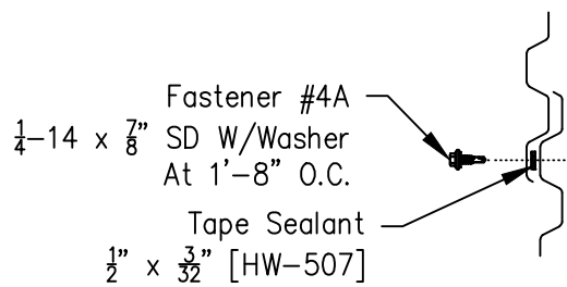
PBD Panel Sidelap
