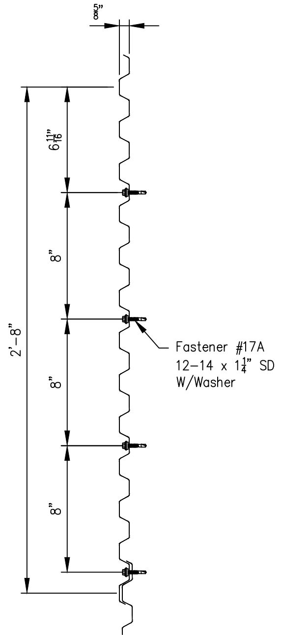
PBD Fastener Location At Intermediate Supports
