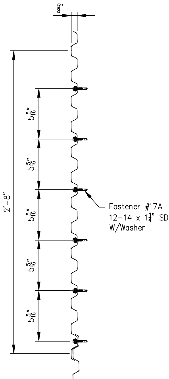
PBD Fastener Location At Panel Ends/Endlaps
