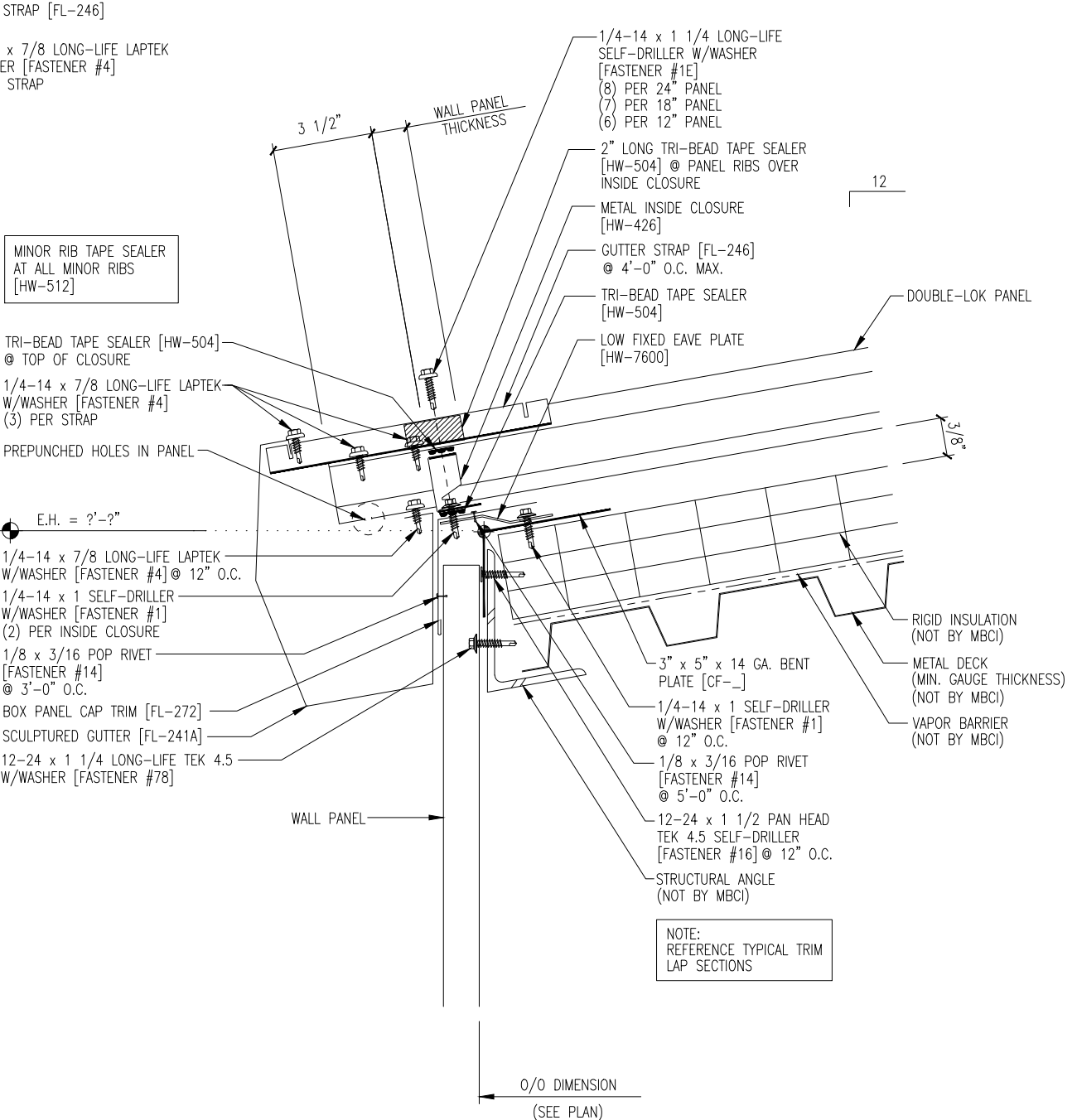
FASTENER SEQUENCE @ EAVE
