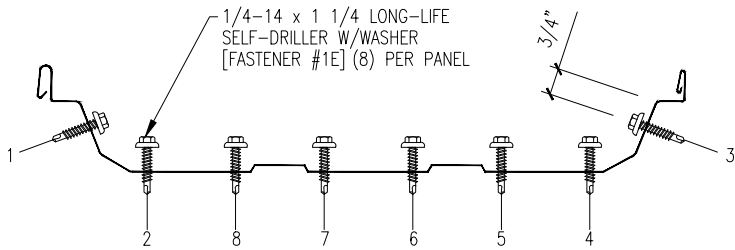
FASTENER SEQUENCE @ EAVE
