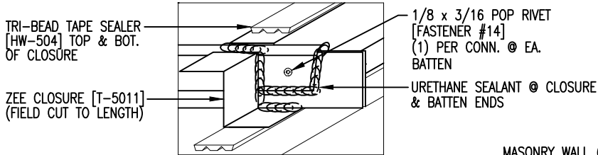
HIGH EAVE SEALANT DETAIL
