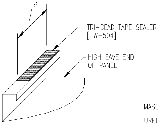
HIGH EAVE SEALANT DETAIL
