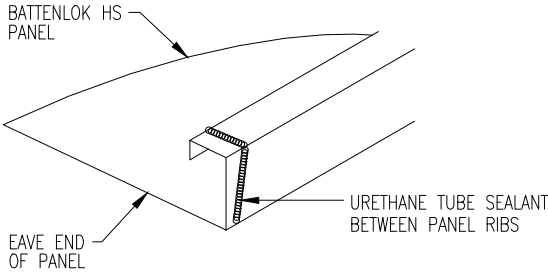
EAVE SEALANT DETAIL
