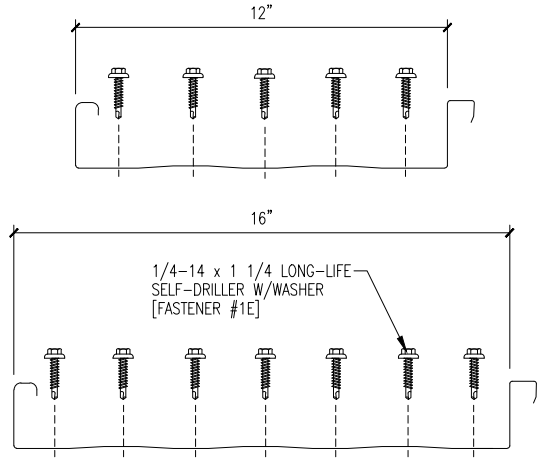
FASTENER LOCATIONS
