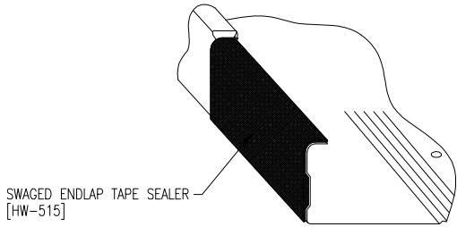
VIEW "A"
