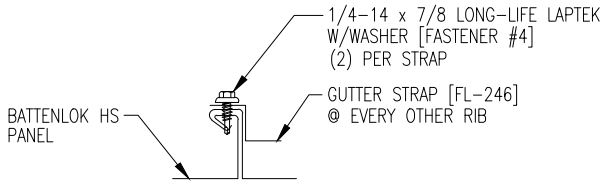
GUTTER STRAP ATTACHMENT
