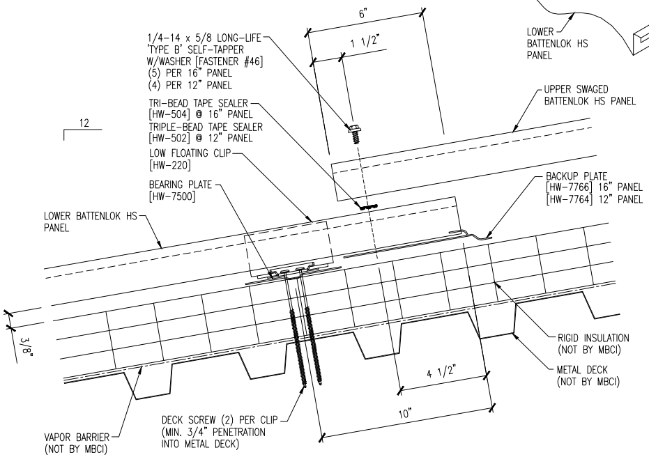
FASTENER INSTALLATION SEQUENCE
