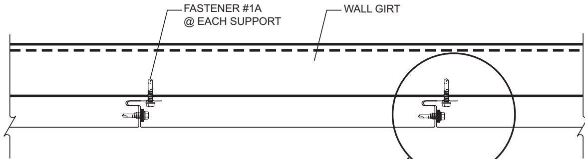
CROSS SECTION OF PANEL ATTACHMENT
