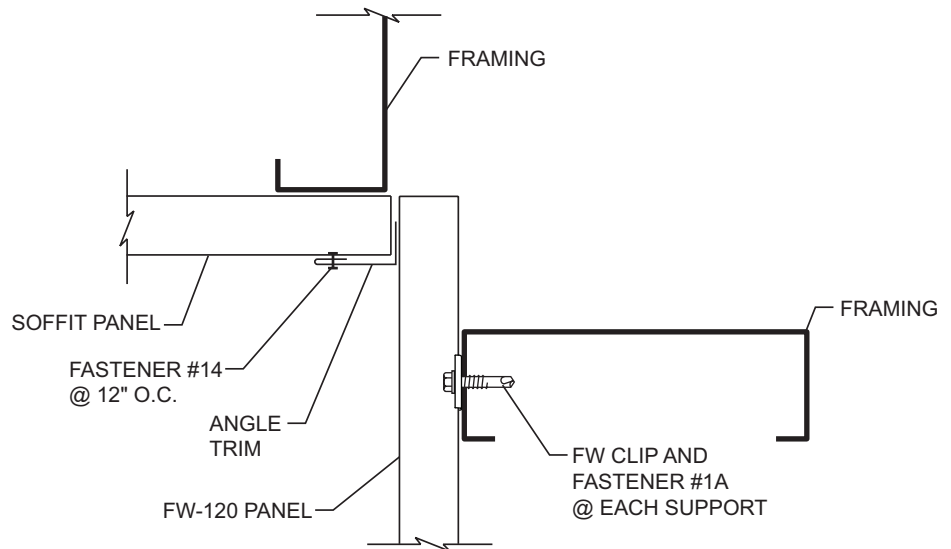
INSIDE SOFFIT-WALL DETAIL
