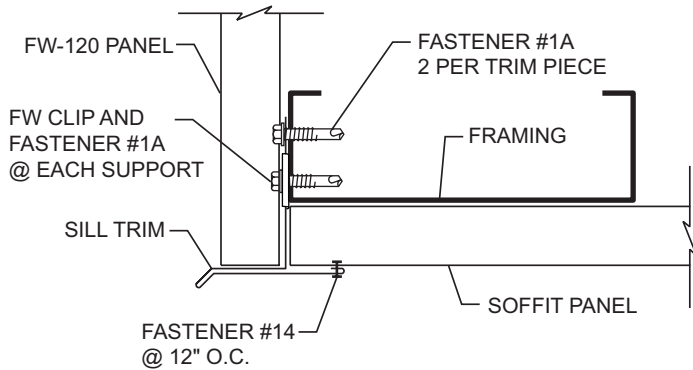
OUTSIDE SOFFIT-WALL DETAIL
