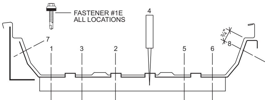
FASTENER SEQUENCE FIRST RUN - ENDLAP
